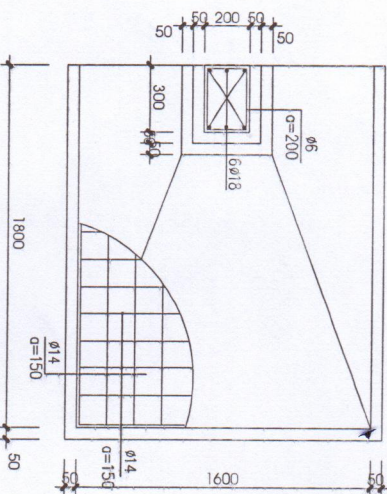
MÓNG MC1 (1/2CK)
